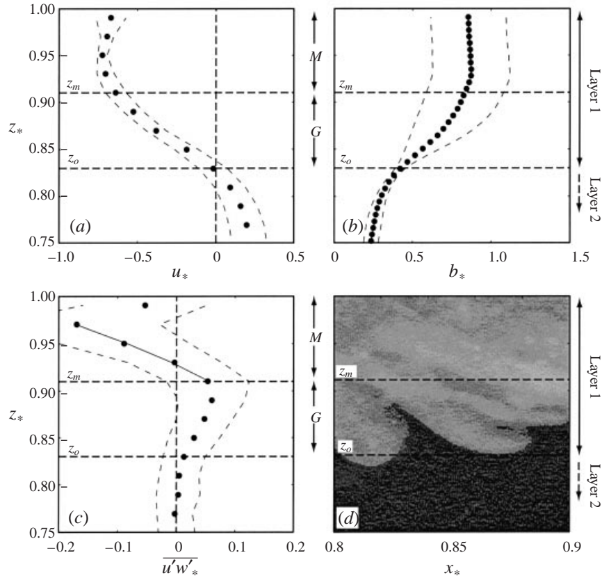
FIGURE 7. Structure of the upper layer shown as profiles of (a) non-dimensional mean horizontal velocity u_* , (b) non-dimensional mean buoyancy b_* , (c) non-dimensional Reynolds stress \overline{u'w'_*} , and (d) a sample photographic image from experiment 5. Thin dashed lines indicate \pm\sigma . Note that only the top quarter of the basin depth is shown here so that the structure of the upper layer may be seen clearly. See text for further details.
